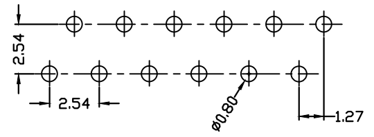
Recommended P.C.B Layout(Top Side)
