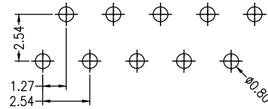
Recommended P.C.B Lavout Top Side)
