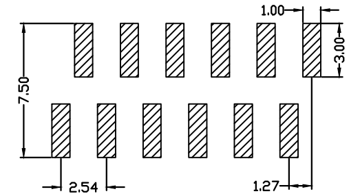
Recommended P.C.B Layout(Top Side)
