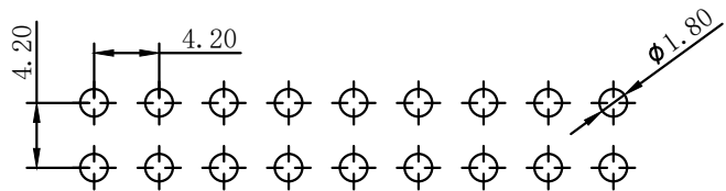
P. C. B LAYOUT
